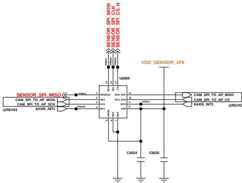
ACC&GYRO SENSOR
