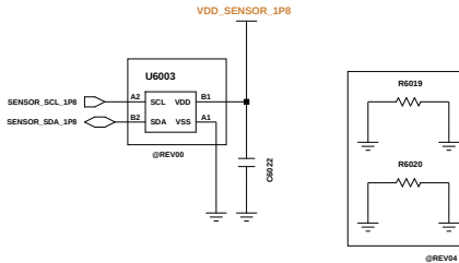
AMBIENT SENSOR MAGNETIC SENSOR
