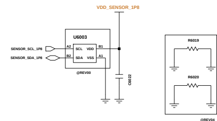
AMBIENT SENSOR MAGNETIC SENSOR
