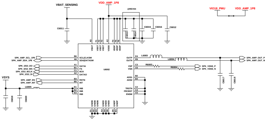
SPK AMP
