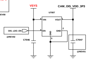
RCAM1_OIS
