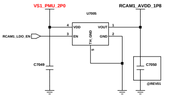
RCAM1_AVDD
