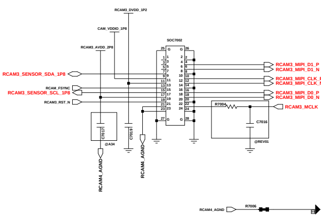
RCAM3_5M_MACRO_CAMERA(24PIN)
