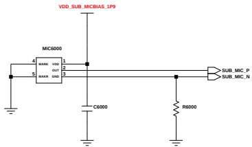
2nd MIC
