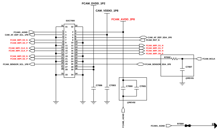
FRONT_13M CAMERA (30PIN)
