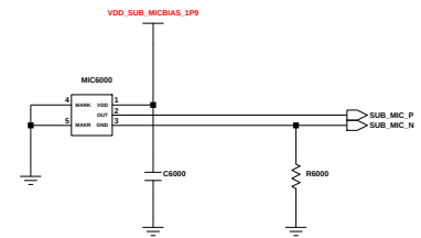
2nd MIC
