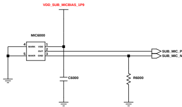
2nd MIC
