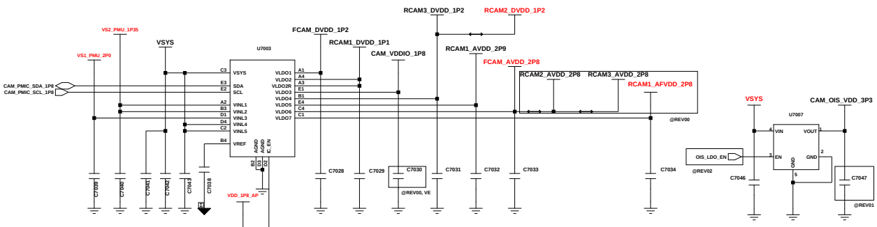
RCAM1_OIS
