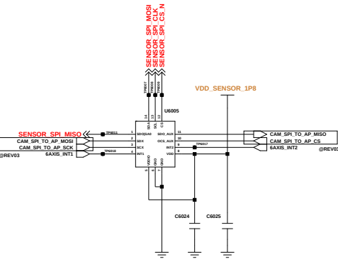
ACC&GYRO SENSOR
