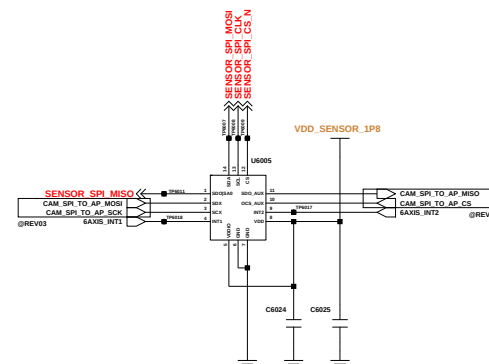
ACC&GYRO SENSOR
