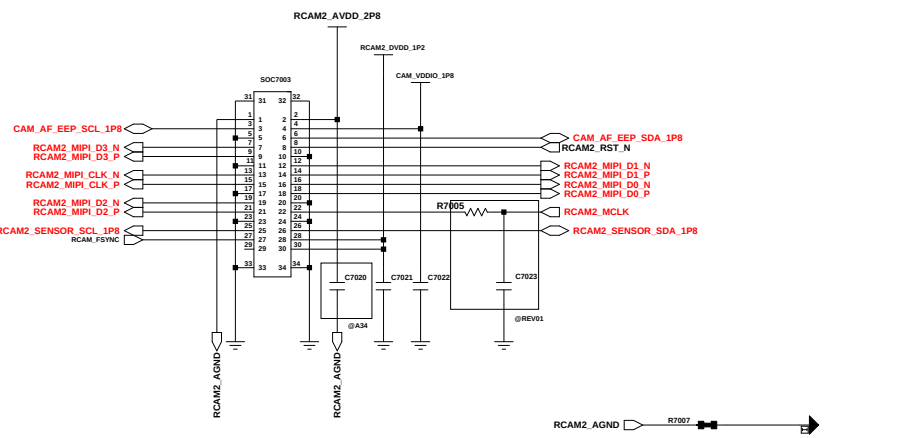
RCAM2_SUPER WIDE_8M CAMERA(30pin)
