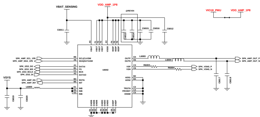
SPK AMP
