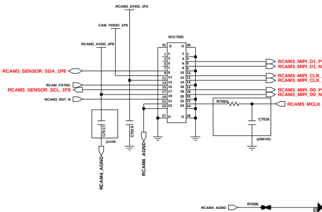
RCAM3_5M_MACRO_CAMERA(24PIN)
