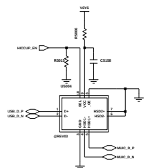
HICCUP SWITCH
